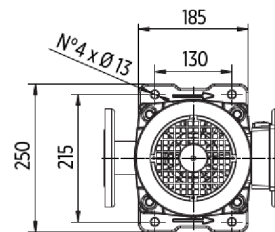
Round flanges on body type PN25/40
