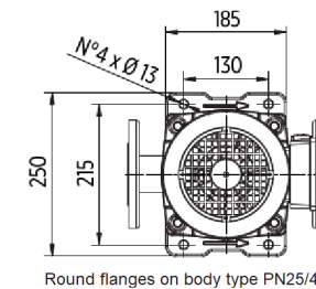
Round flanges on body type PN25/40
